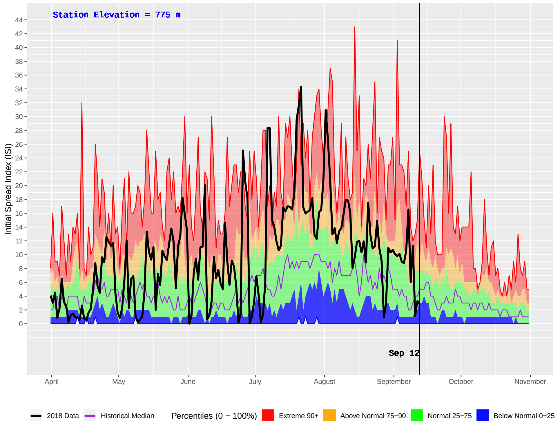
ELKO (412) : Historical (1970–2016) and Current (2018) Daily Initial Spread Index (ISI)
